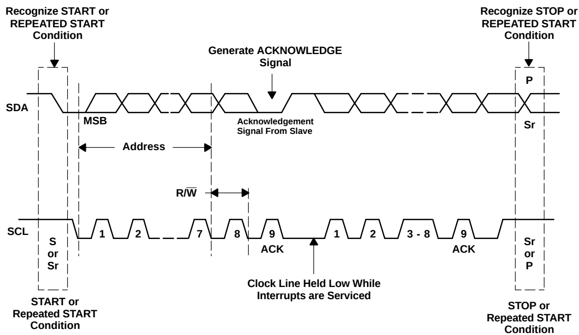
Figure 31. Bus Protocol
