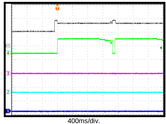
PMAX Limit Triggered (10)
