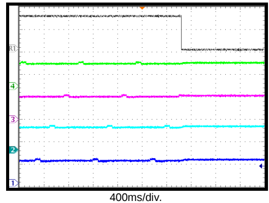
Shutdown through EN No PD connection
