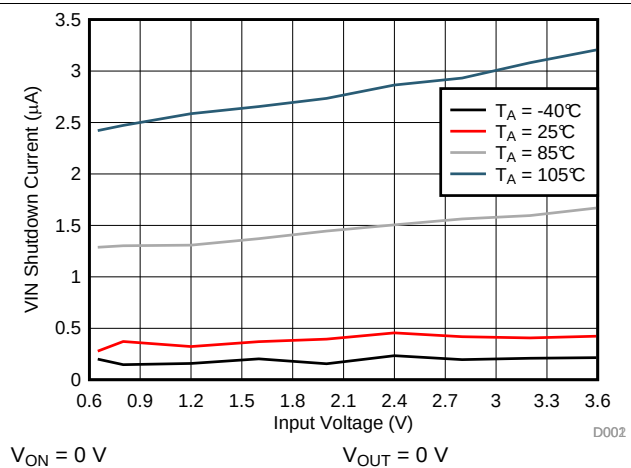
Figure 4. Input Shutdown Current vs Input Voltage
