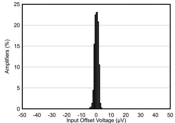
图 8-2. OPAx205 e-trim™ Operational Amplifier Offset
