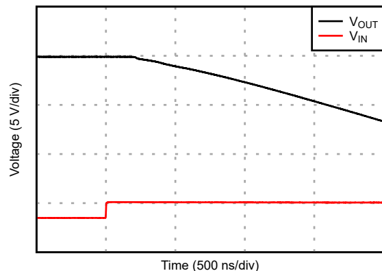
图 6-35. Positive Overload Recovery, Gain = -1
