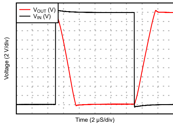
图 6-41. Large-Signal Step Response, Gain = -1
