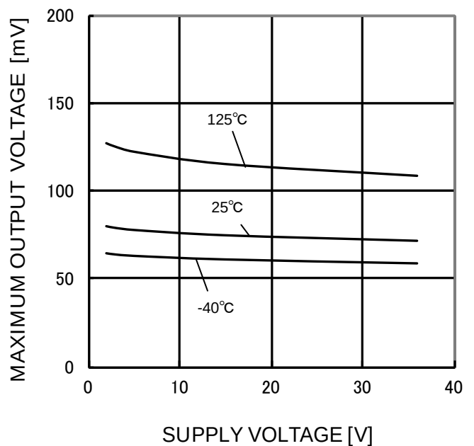
Figure 28. Maximum Output Voltage – Supply Voltage ( I_{\text{sink}}=4\text{mA} )
