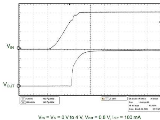
Figure 28. Start-up transient
