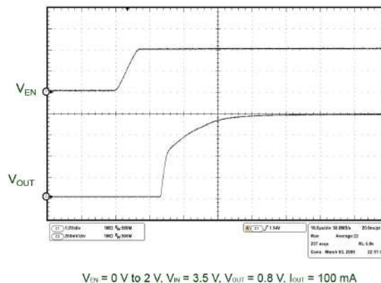
Figure 29. Enable transient
