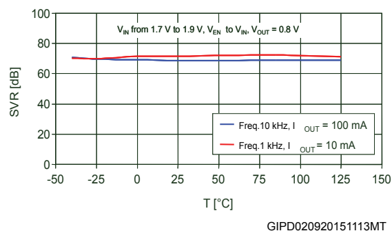
Figure 17. Supply voltage rejection vs. temperature ( V_{OUT} = 0.8 V)
