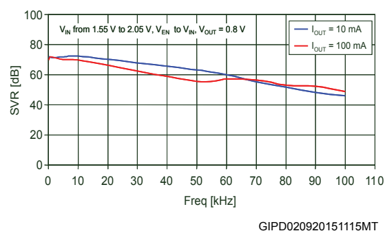
Figure 19. Supply voltage rejection vs. frequency ( V_{OUT} = 0.8 V)
