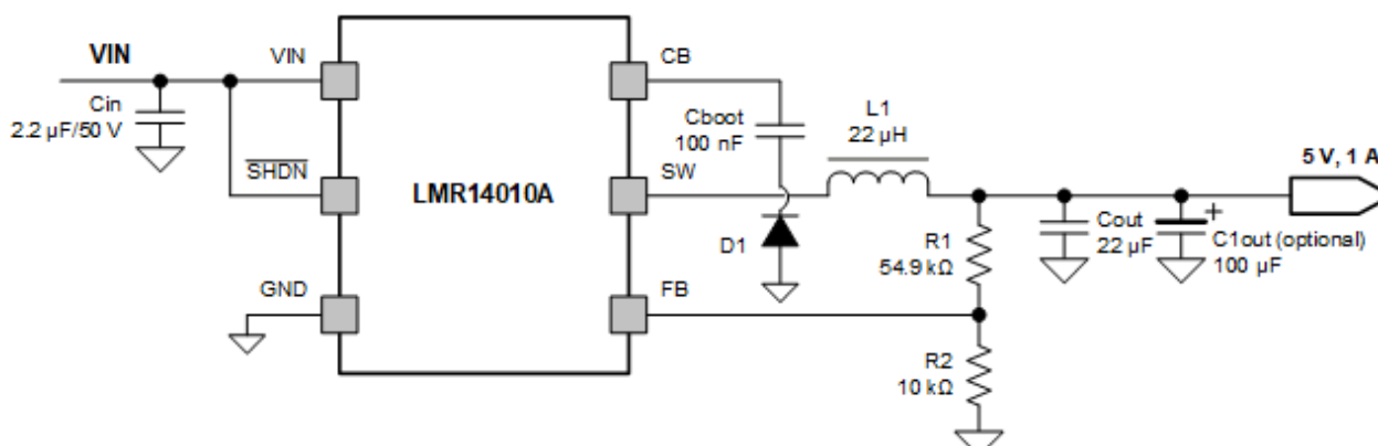
图 7-1. LMR14010A Application Circuit, 5-V Output
