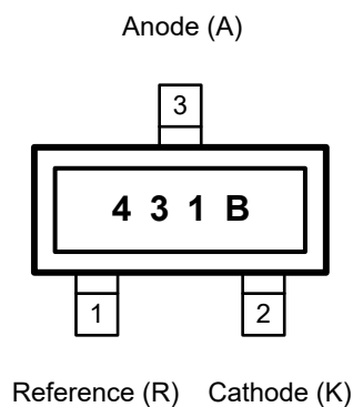
CJ431B SOT-23 Package
