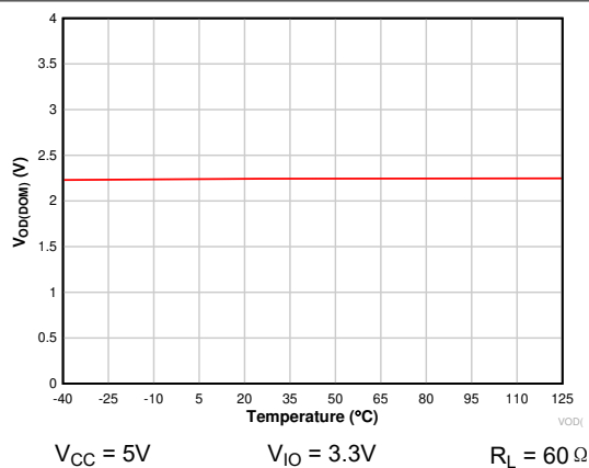
图 6-1. V_{OD(DOM)} vs Temperature
