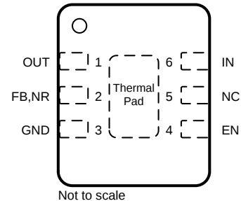
DRV Package 6-Pin WSON With Exposed Thermal Pad Top View
