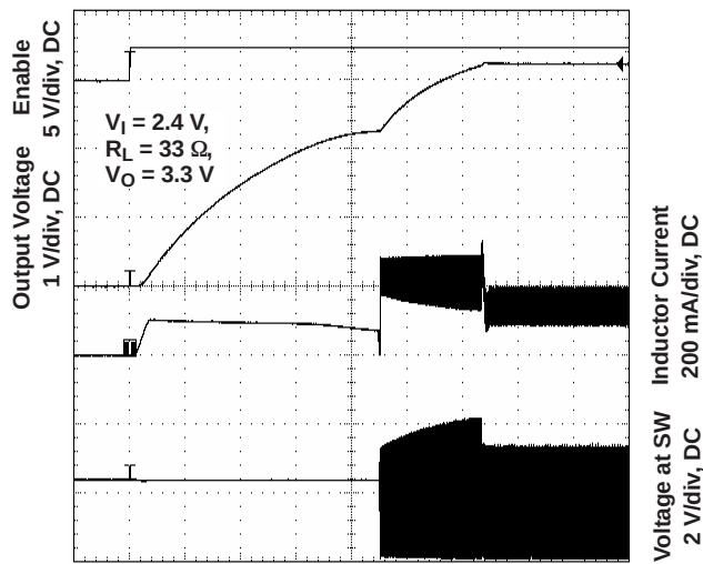
TPS61071 START-UP AFTER ENABLE
