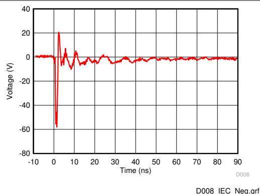
图 5-8. -8kV IEC 61000-4-2 Clamping Voltage Waveform, IO Pin to GND
