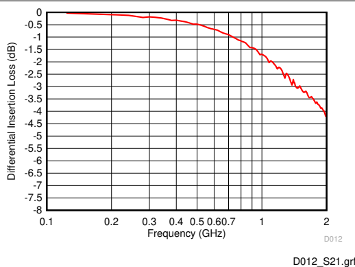
图 5-12. Differential Insertion Loss vs. Frequency
