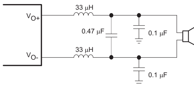
Figure 31. Typical LC Output Filter, Cutoff Frequency of 27 kHz
