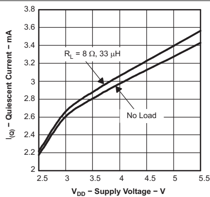
Figure 5. Quiescent Current vs Supply Voltage
