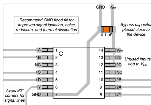
Figure 11. Example layout for the SN74HCS21
