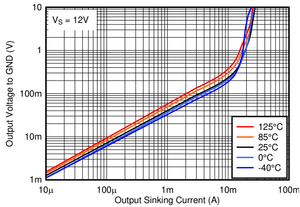
图 6-21. Output Low Voltage vs. Output Sinking Current at 12V
