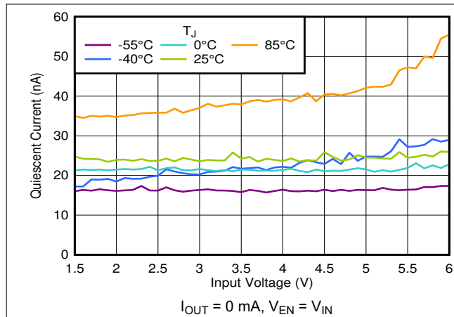
图 6-1. I_Q vs V_{IN} and Temperature
