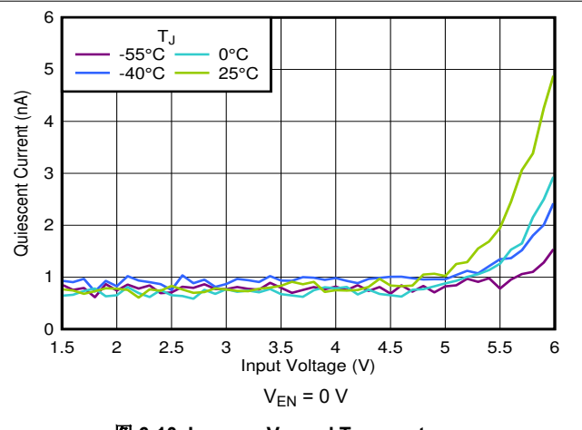
图 6-10. I_{SHDN} vs V_{IN} and Temperature
