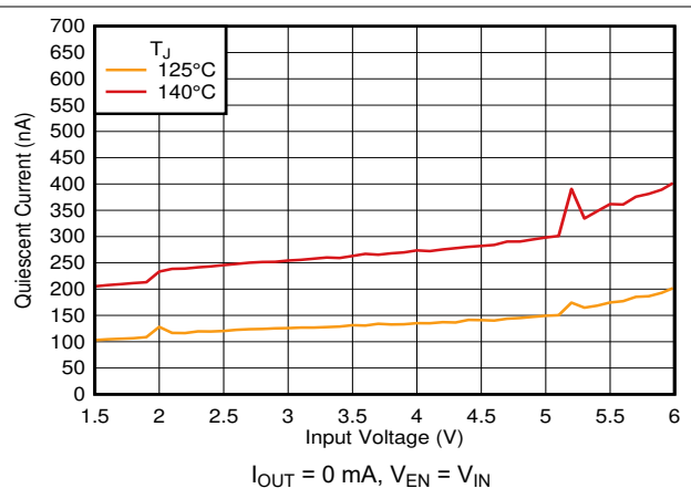
图 6-2. I_Q vs V_{IN} and Temperature
