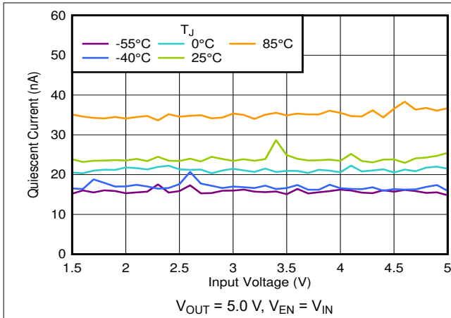
图 6-7. I_Q in Dropout vs V_{IN} and Temperature
