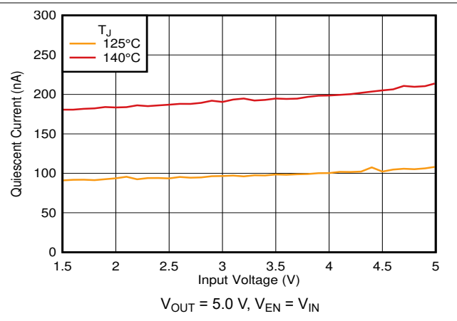
图 6-8. I_Q in Dropout vs V_{IN} and Temperature
