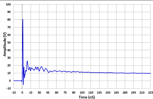
图 5-1. IEC 61000-4-2 Clamp Voltage +8 kV Contact ESD
