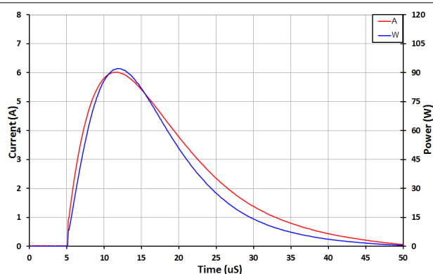
图 5-7. Negative Surge Waveform 8 to 20 \mu s
