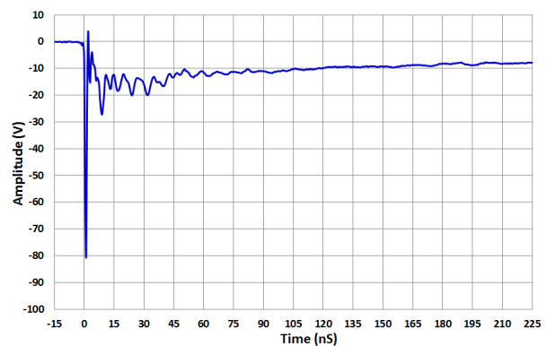
图 7-3. IEC 61000-4-2 Clamp Voltage -8 kV Contact ESD
