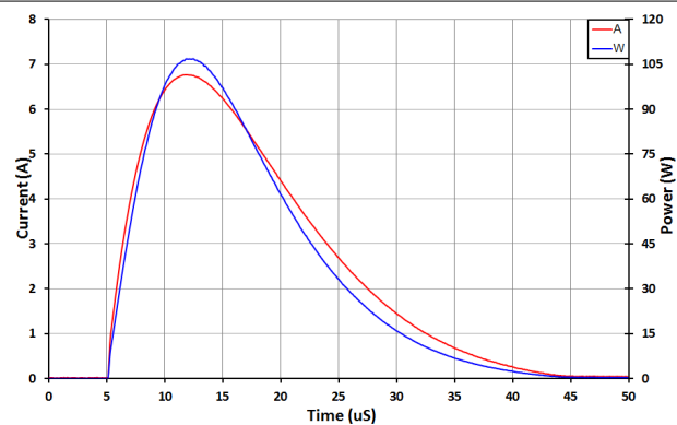
图 5-6. Positive Surge Waveform 8 to 20 \mu s
