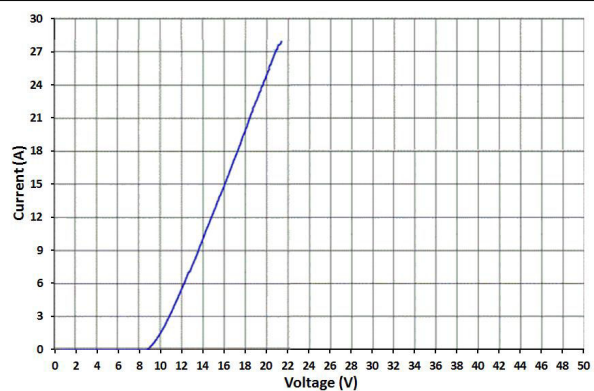
图 5-4. Transmission Line Pulse (TLP) Waveform Pin 2 to Pin 1
