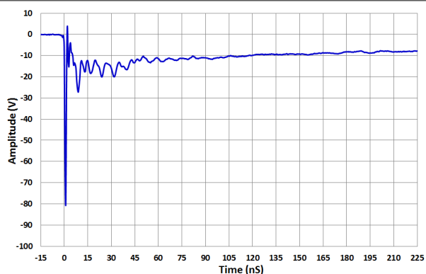
图 5-2. IEC 61000-4-2 Clamp Voltage -8 kV Contact ESD
