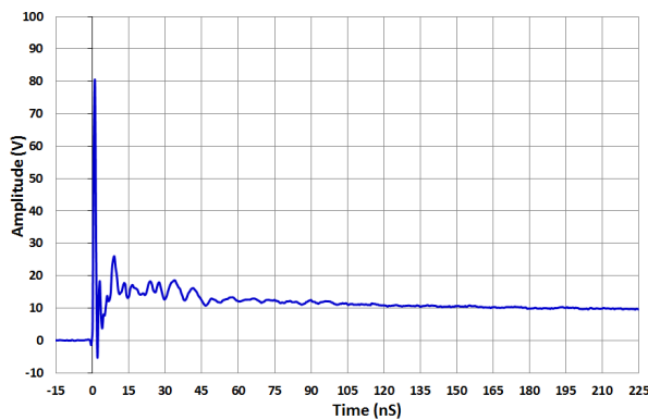
图 7-2. IEC 61000-4-2 Clamp Voltage +8 kV Contact ESD
