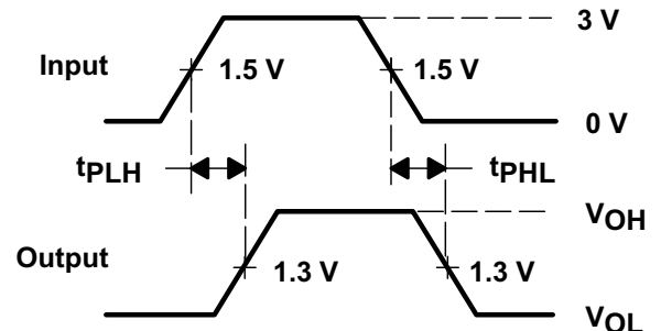
VOLTAGE WAVEFORMS
