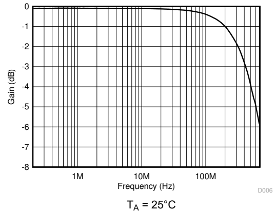
图 6-6. Frequency Response
