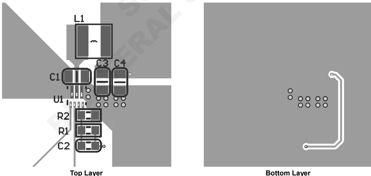
Figure 4. PCB Layout
