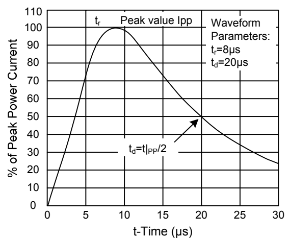
Figure 2. Pulse Waveform
