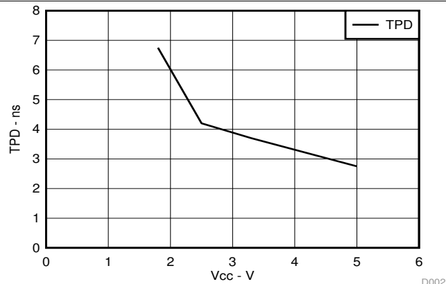
Figure 1. Across Vcc at 25°C
