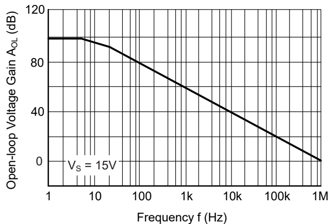
Figure 6-2. Large-Signal Open Loop Voltage Gain
