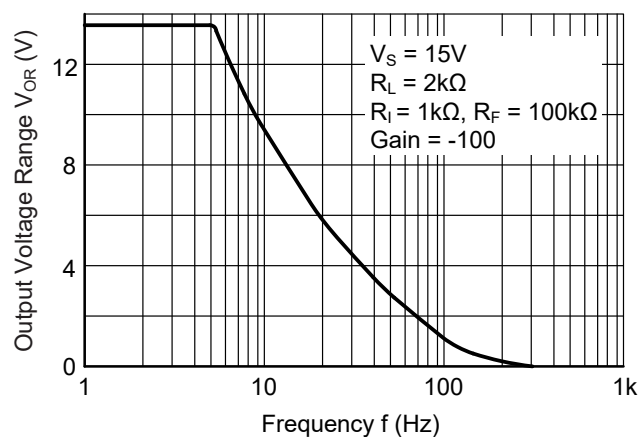
Figure 6-3. Large-Signal Frequency Response
