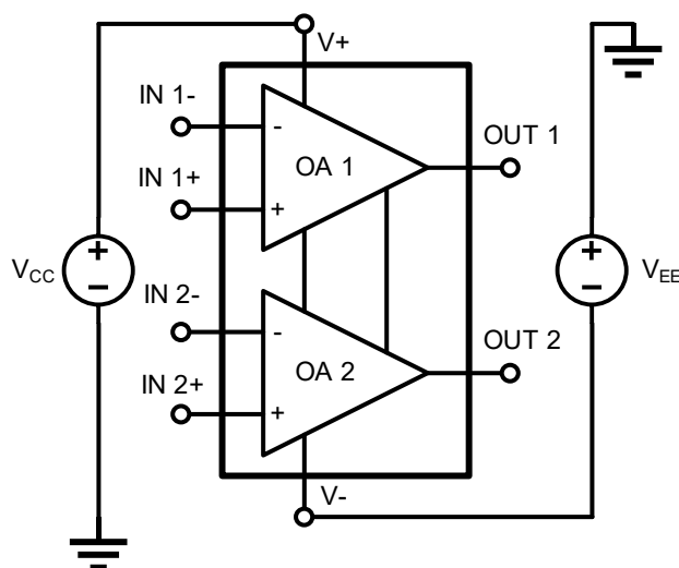
Figure 8-3. Dual Power Supply
