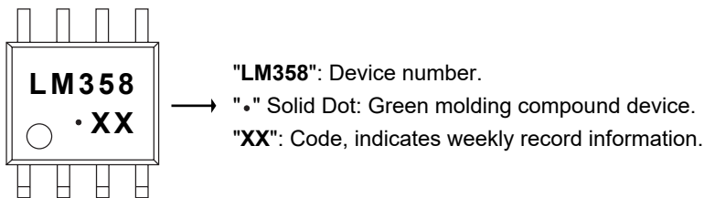
Figure 2-2. Marking Information
