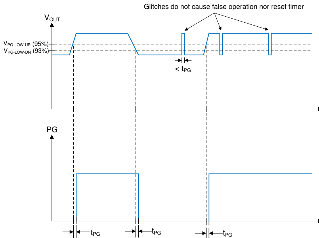
图 8-2. Power-Good-Timing Behavior
