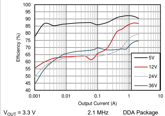
图 9-12. Efficiency
