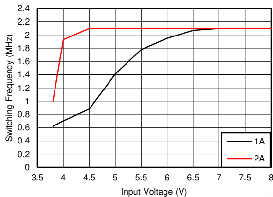
图 8-11. Typical Switching Frequency in Dropout Mode V_{OUT} = 3.3\text{ V} , f_{SW} = 2.1\text{ MHz}
