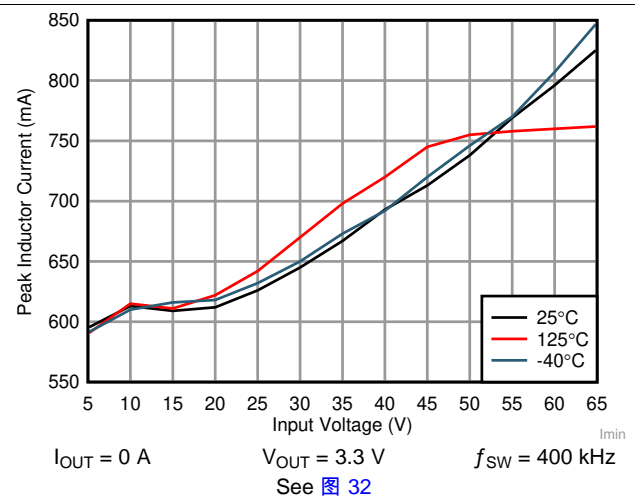
图 2. IPEAK-MIN
