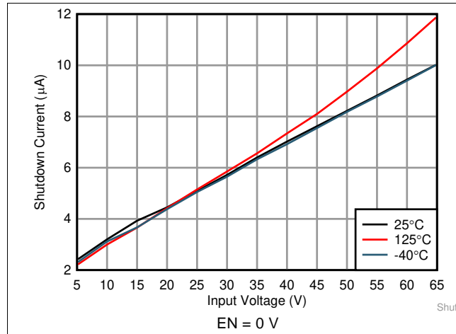
图 1. Shutdown Supply Current
