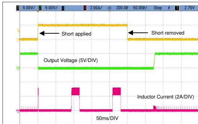
图 7. Short-Circuit Transient and Recovery
