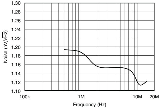
CW INPUT-REFERRED NOISE vs FREQUENCY
