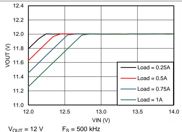
Figure 18. Dropout Curve
