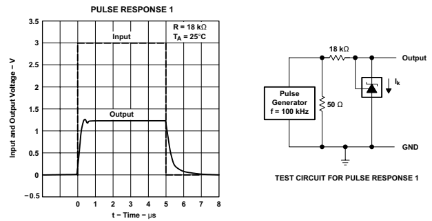
图 5-12. Pulse Response 1
