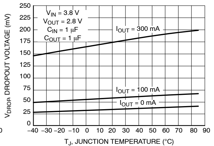
Figure 14. Dropout Voltage vs. Temperature V OUT = 2.8 V (UDFN)
