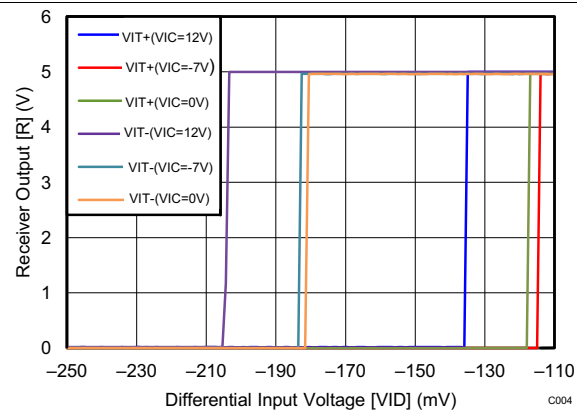
Figure 4. Receiver Output vs Differential Input Voltage
