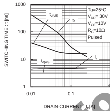
Fig.12 Switching Characteristics
