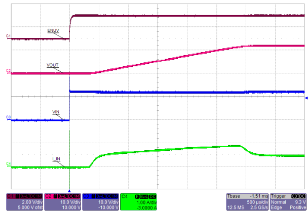
Figure 37. Hot-Plug Start-Up: Output Ramp With 24 Ω Load at Start Up
