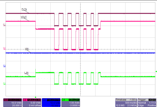
Figure 39. Overvoltage Recovery
