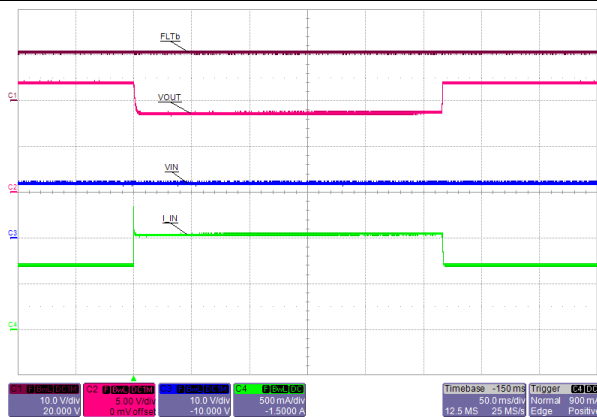
Figure 38. Overvoltage Shutdown
