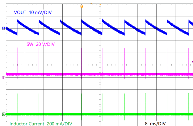
LMR38010 V_{OUT} = 5\text{ V} No Load AC Coupled
