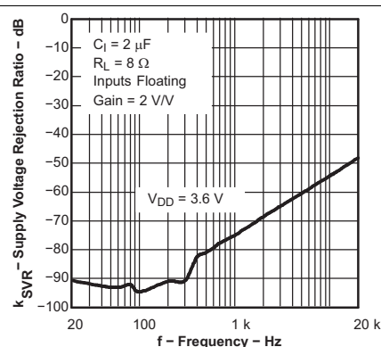
Figure 26. Supply Voltage Rejection Ratio vs Frequency
