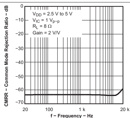
Figure 30. Common-mode Rejection Ratio vs Frequency
