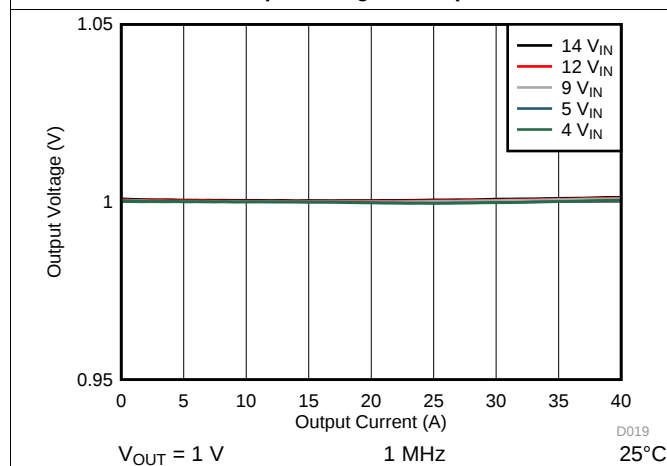
图 9. Output Voltage vs Output Current
