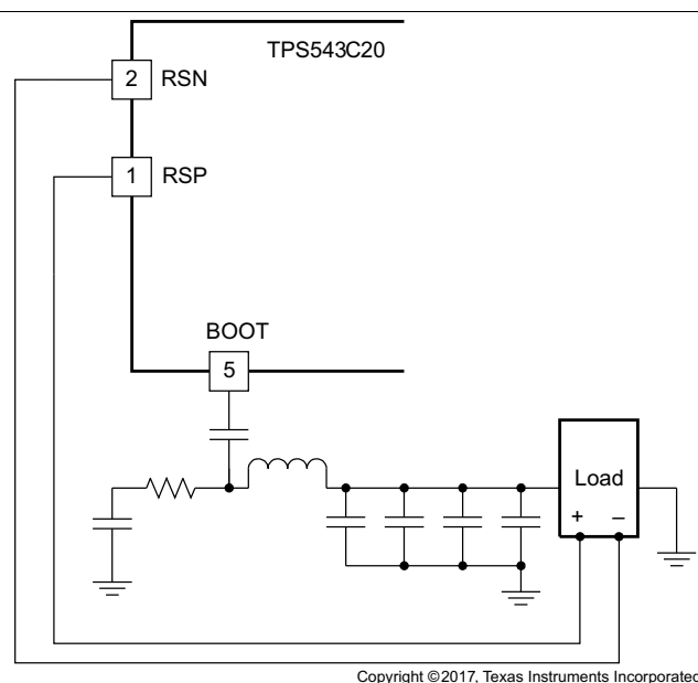
图 23. Remote Sensing Without Feedback Resistors
