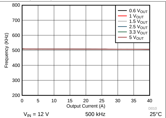
图 8. Switching Frequency vs Output Current
