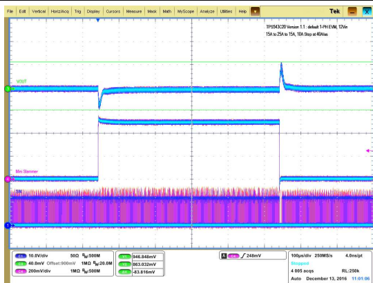
Figure 26. Transient Response of 0.9-V Output at 12-V IN , Transient is 15 A to 25 A to 15 A, the Step is 10 A at 40 A/μs
