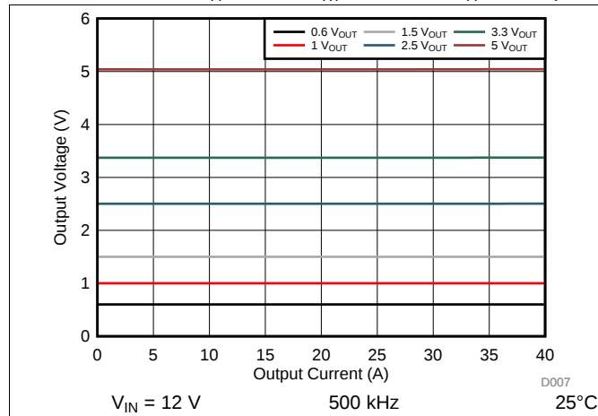
图 7. Output Voltage vs Output Current
