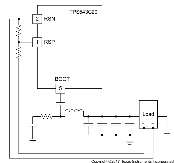
图 22. Remote Sensing With Feedback Resistors
