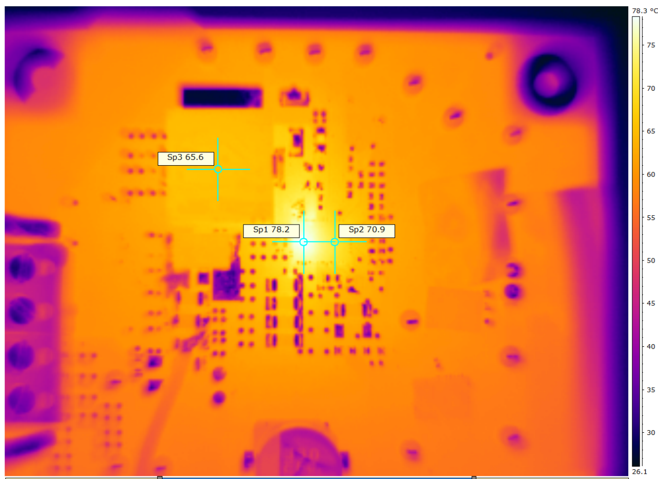
图 45. Thermal Image at 0.9-V Output at 12 VIN, 40-A Output, at 25°C Ambient
