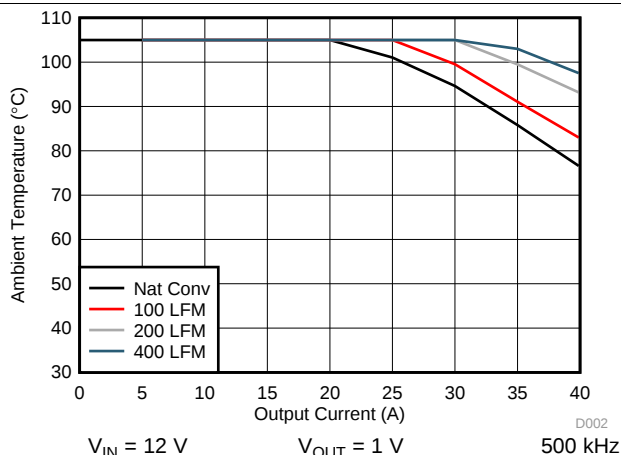
图 44. Safe Operating Area
