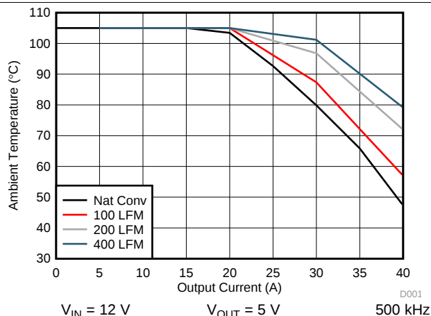
图 43. Safe Operating Area
