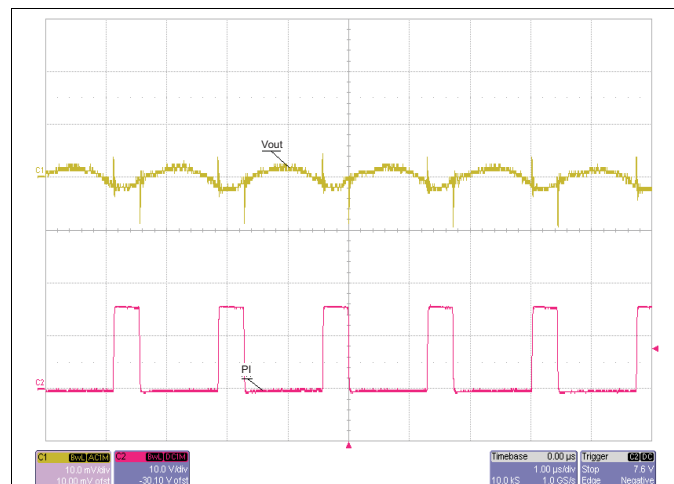
Figure 17. Output Ripple
