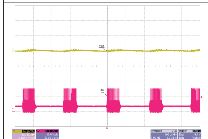
Figure 21. Eco-mode
