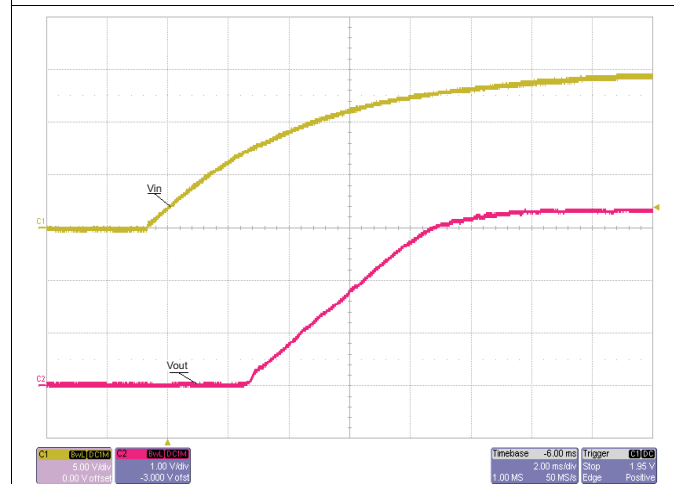
Figure 19. Startup
