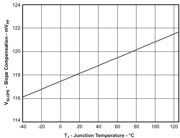
图 7-10. Current Slope Compensation Voltage vs Temperature
