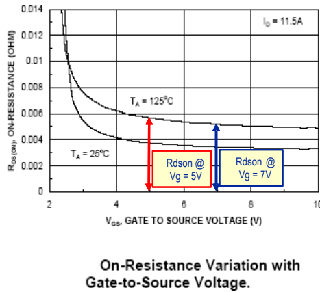
图 7-2. R_{DS(on)} of MOSFET as Function of V_{GS}
