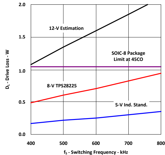
图 7-3. Drive Power as Function of V_{GS} and F_{sw}
