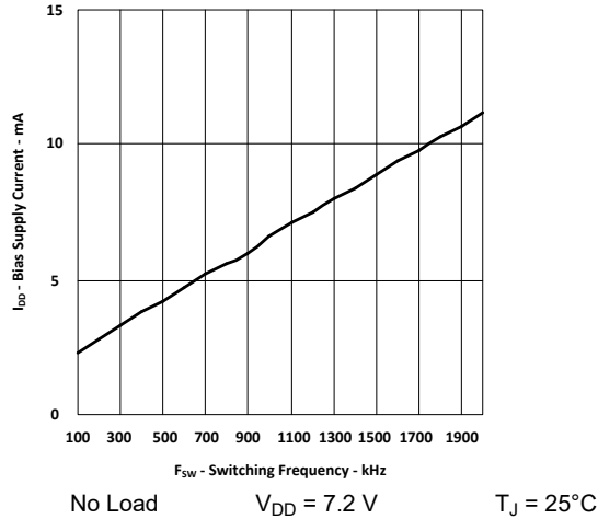
图 5-14. Bias Supply Current vs Switching Frequency
