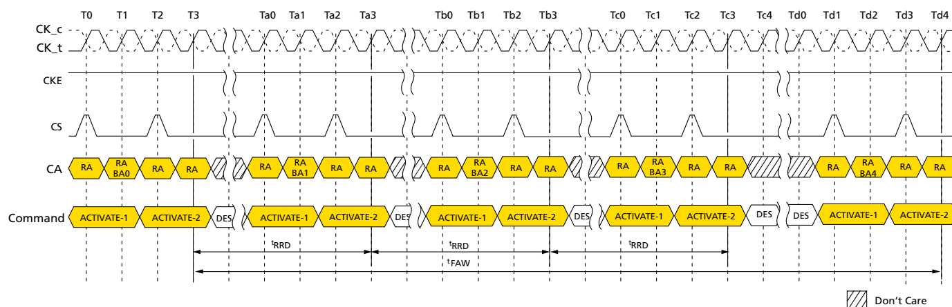
Figure 15: t_{FAW} Timing
