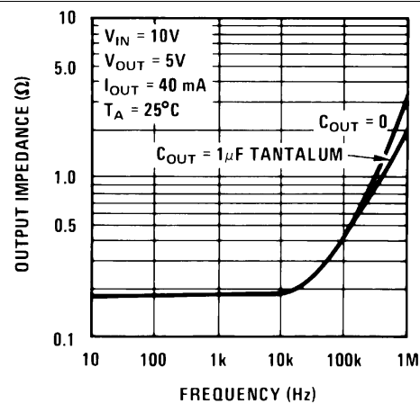
Figure 5. Output Impedance
