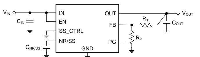
图 38. Adjustable Operation
