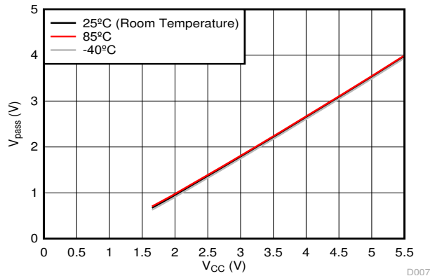
图 8-2. Pass-Gate Voltage ( V_{pass} ) vs Supply Voltage ( V_{CC} ) at Three Temperature Points
