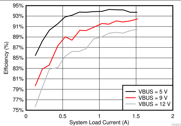
图 7-2. System Light Load Efficiency vs System Light Load Current
