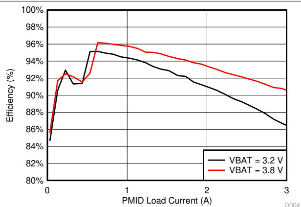
图 7-3. Boost Mode Efficiency vs PMID Load Current
