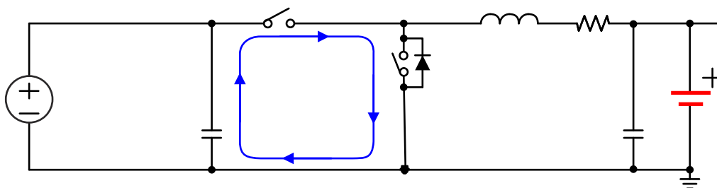
图 11-1. High Frequency Current Path
