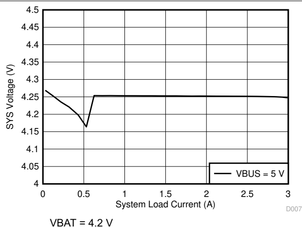
图 7-6. SYS Voltage Regulation vs System Load Current
