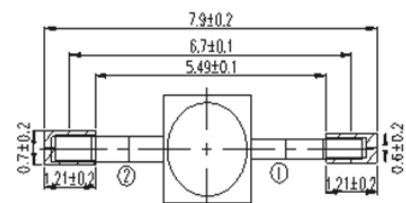
Recommend Soldering Pad
