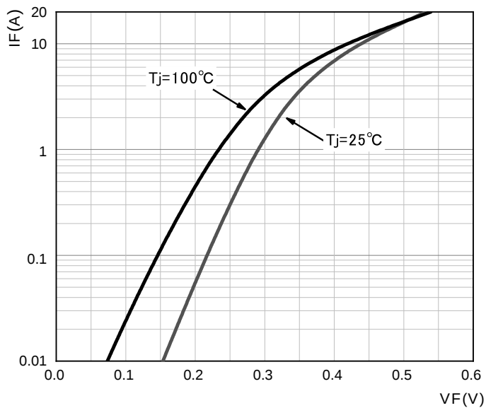
FIG.3: INSTANTANEOUS FORWARD CHARACTERISTICS
