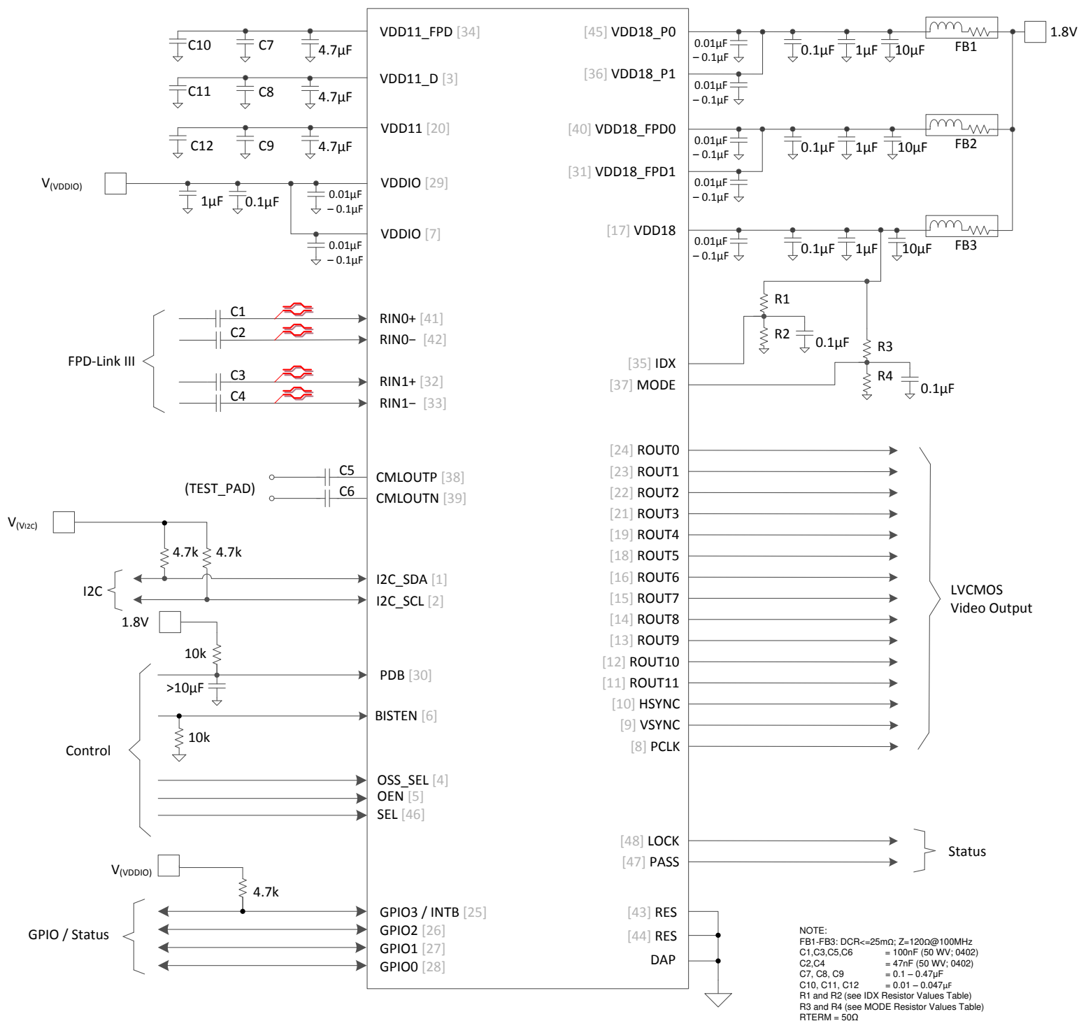
图 6-4. Typical Connection Diagram STP
