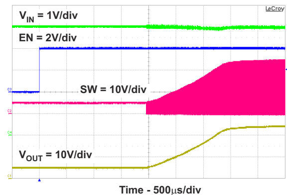
图 8-8. Start-Up
