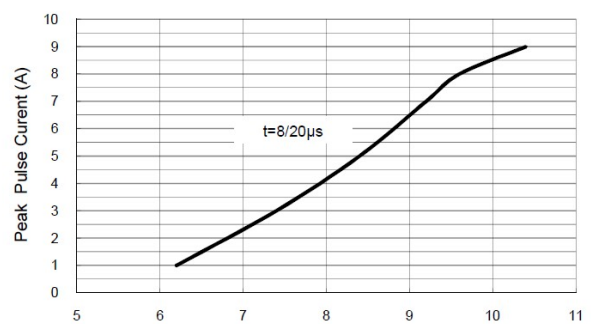
Fig 6 Clamping Voltage vs Peak Pulse Current
