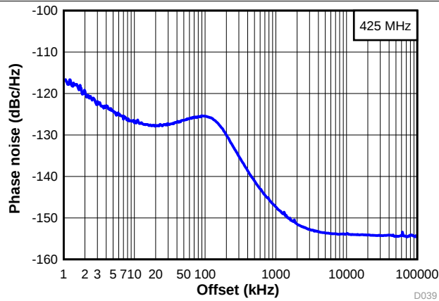
图 9. Wide Band Phase Noise at 425 MHz
