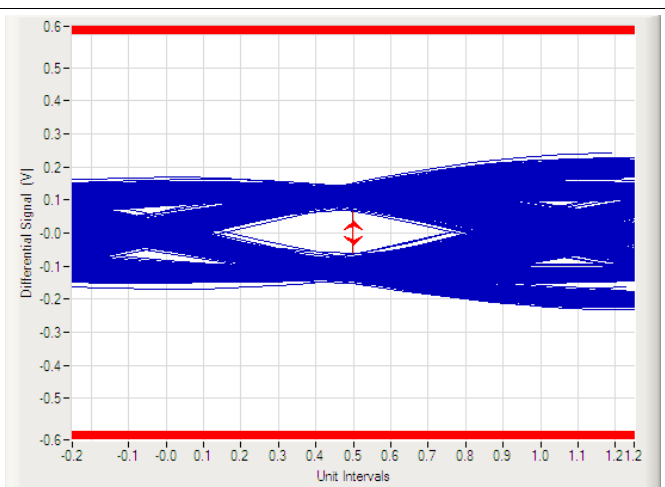
Figure 15. USB 3.1 Gen 2 10-Gbps Eye Diagram (with TPD1E01B04)
