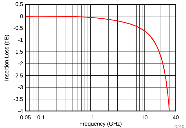
Figure 10. Insertion Loss
